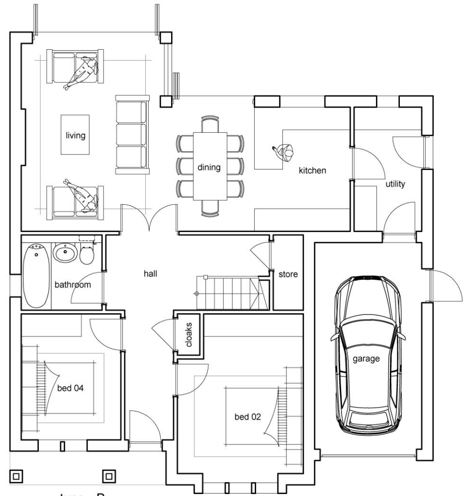
type - B 931 sq ft ground floor plan
