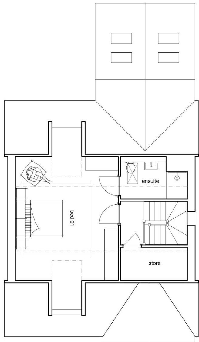
type - A 462 sq ft first floor plan
