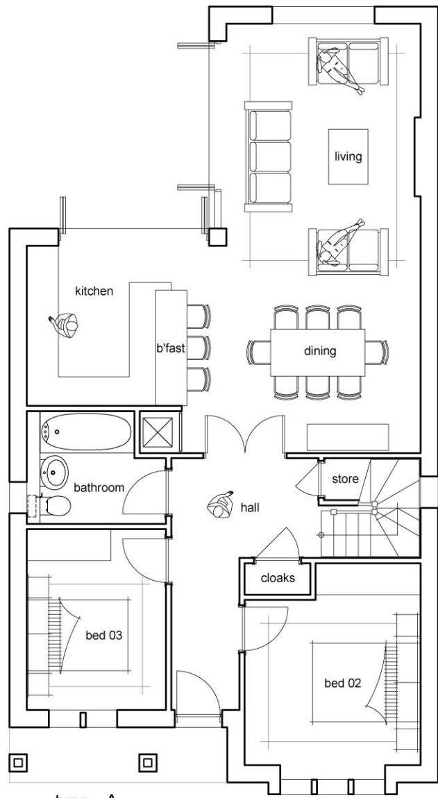
type - A 925 sq ft ground floor plan
